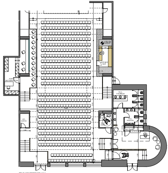
ZEUS CONFERENCE HALL 424.7 m 2 H=3.70 m. 460 SEATS SCALE 1:100
