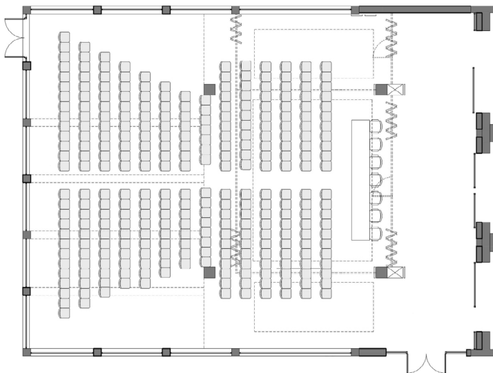
SELENA CONFERENCE HALL 322.5 m 2 H = 2.70 m
